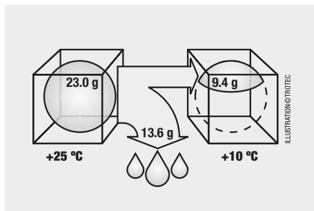
Figure 1: Water vapour content of the air [8]
