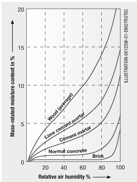
Figure 19: Sorption isotherms for various building materials [19]
