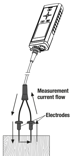
Figure 9: Sketch of resistance measurement with the T3000
