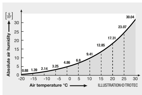
Figure 2: Saturation curve
