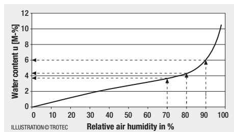
Figure 37: Example of determination of the water content according to the hygrometric method by means of the sorption isotherm.
