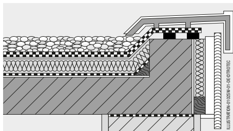
Figure 29: Flat roofs (thermal roof), insulated
