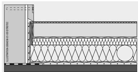
Figure 28: Fabricated floor with footstep sound insulation
